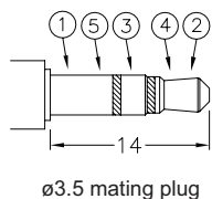
3.5 mating plug
