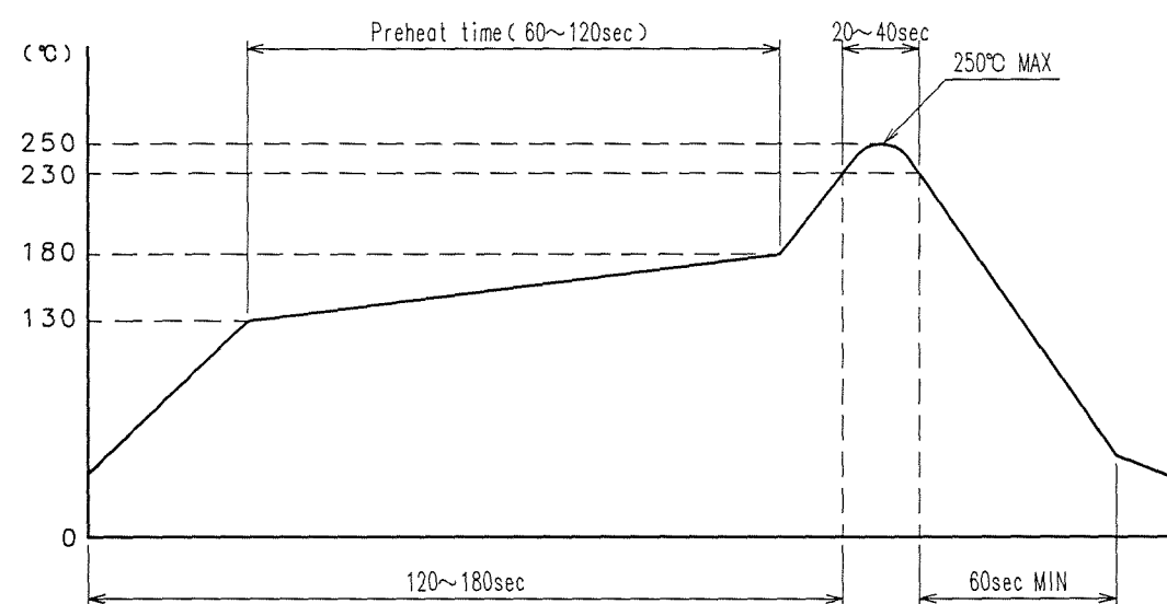
Recommended temperture profile for reflow
