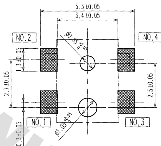
Recommended PC board pattern.
