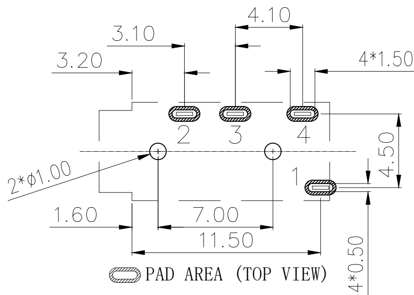
RECOMMEND PCB LAYOUT(±0.05)
