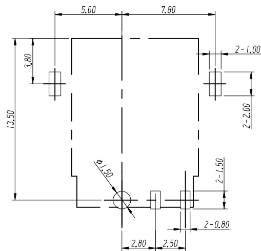
PCB LAYOUT TOP VIEW (TOLERANCE:±0.05)
