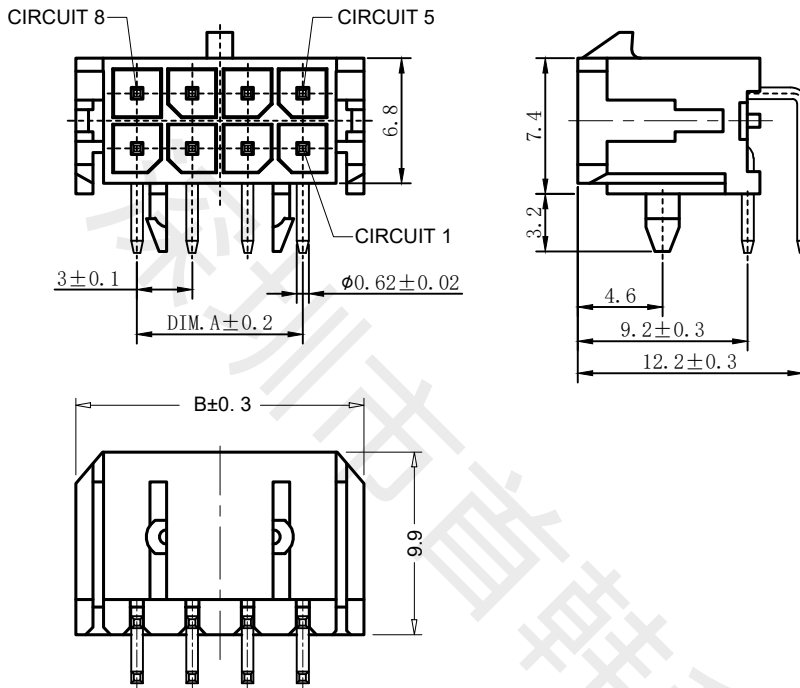
CIRCUIT SIZE LAYOUT
